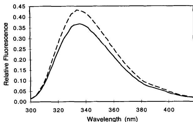
Fig. 2. Tryptophan fluorescence emission spectra of recombinant PEDF in the absence (solid line) and presence (dashed line) of heparin. PEDF, 0.7 \mu M, was in 20 mM sodium phosphate, pH 7.4. Upon addition of an excess of heparin, sufficient to saturate the heparin binding site (15 \mu M) an approximately 17% enhancement in fluorescence resulted, but without change in shape of the curve or the position of the maximum.
